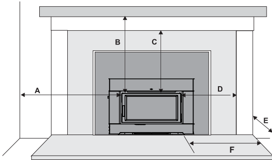
Clearance diagram for Installations
